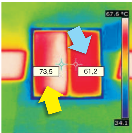
Figura 1 Silox putz 2D nero e Silox putz riflex 2D nero
